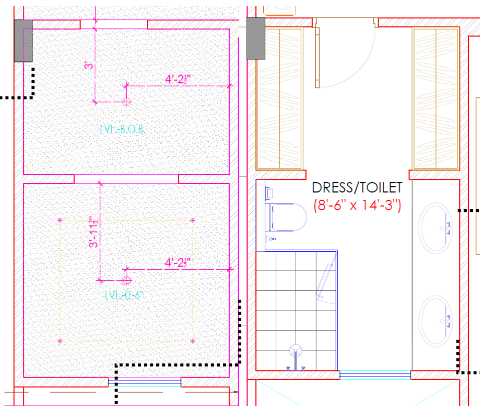
WASHROOM OPT.-01
