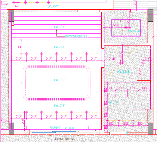
CEILING PLAN
