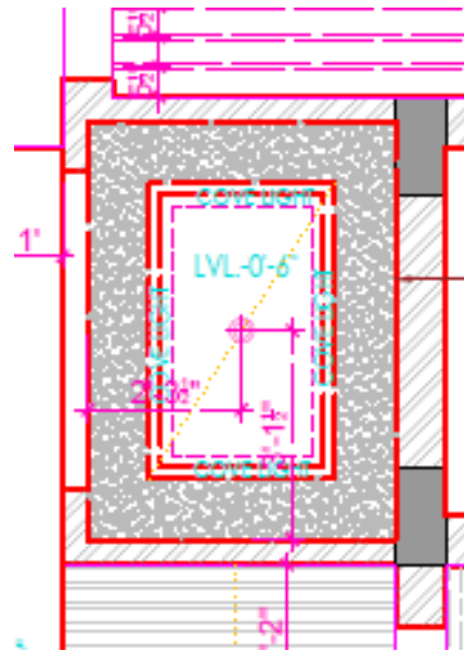
CEILING PLAN
