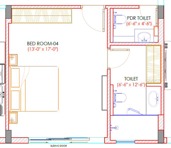
BEDROOM LAYOUT PLAN
