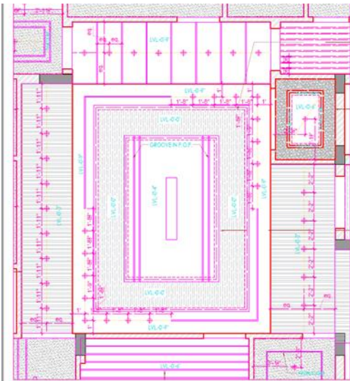
CEILING PLAN
